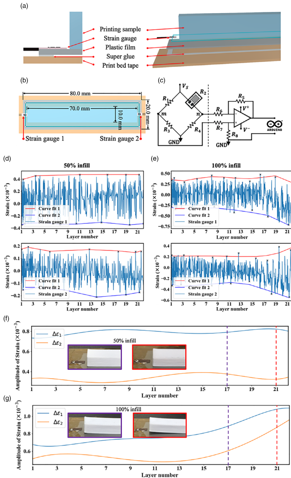
Figure 2. a) The sectional and exploded view of strain gauge setup. b) The physical dimension of the plastic film and printing sample. c) Circuit for strain gauge measurement, where Wheatstone bridge is on the left and LM741 amplifier is on the right. d,e) Results of strain against layer number plots for 50% and 100% infill printing sample. Red and blue curves are polynomial fitting of the boundary of strain data. f,g) Plots for amplitude of strain against layer number with the view of printing sample condition at layer 17 and layer 21 for 50% and 100% infill prints.
