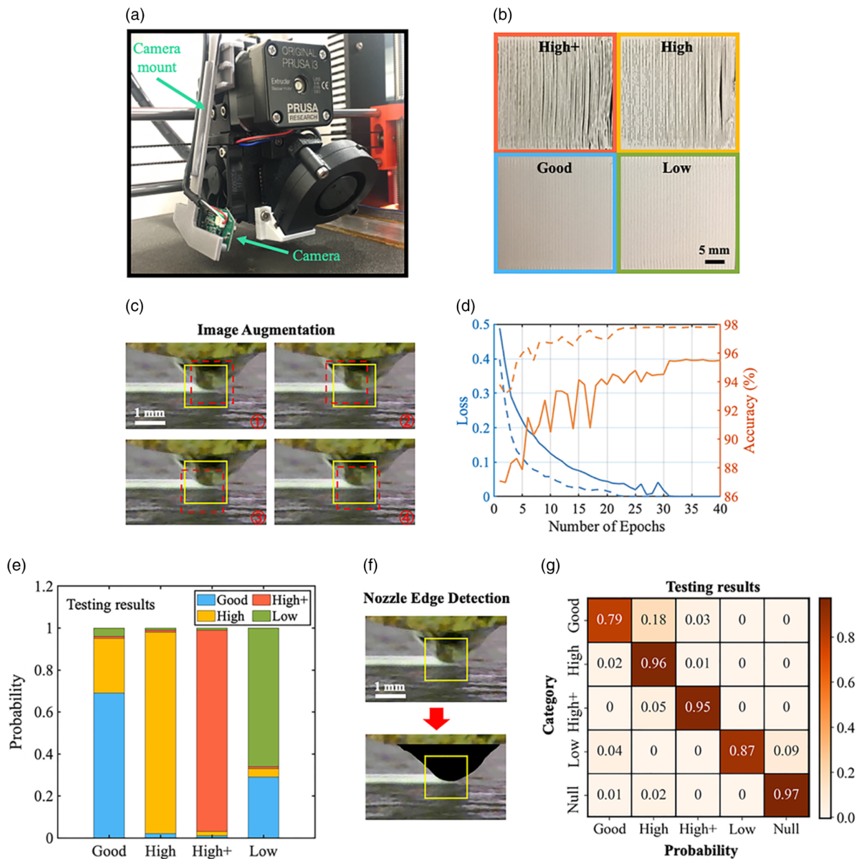
Figure 1. a) Monitoring system where a camera is attached to the mount in-house designed and 3D printed. b) Images for four cases which represent the four conditions of nozzle height. c) Image collection and augmentation where yellow box is the area of interest and red dash box is the actual extracting location. d) Training result of the CNN algorithm based on validation data set. The accuracy converges to 95.5% for the first model (solid line) and 97.8% for the enhanced model (dashed line). e) The bar plot presenting probability distribution for each category of the testing data set. f) Nozzle edge detection and masking the corresponding area in black color. g) The confusion matrix showing testing data set accuracy for each category.
